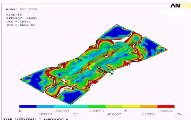
Fig 6. Dynamic simulating, moments at 50.
