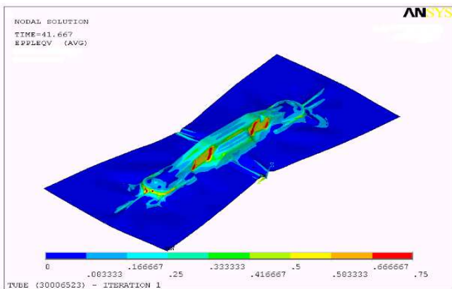
Fig 5. Dynamic simulating, moments at 40.
