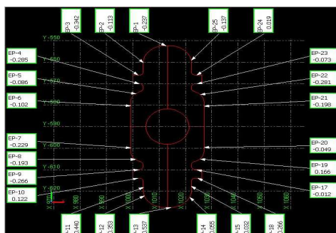
Fig 4. The Deviation of the Sizes from the Nominal Value.
