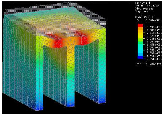
Fig 1. Solicitations and tensions in critical zone of component elements.
